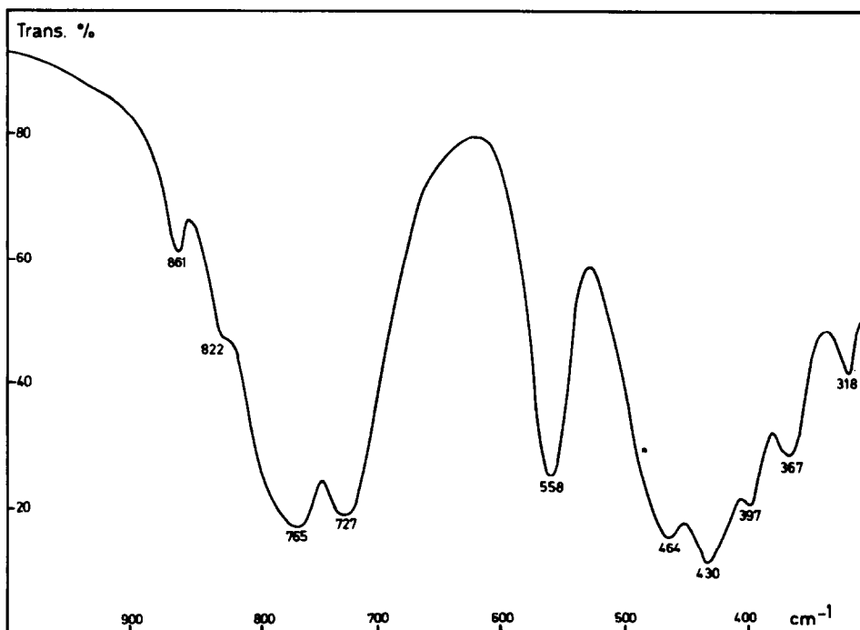
FIG. 5. Infrared spectrum of Pb_2Sc_2Ge_2O_9 .
