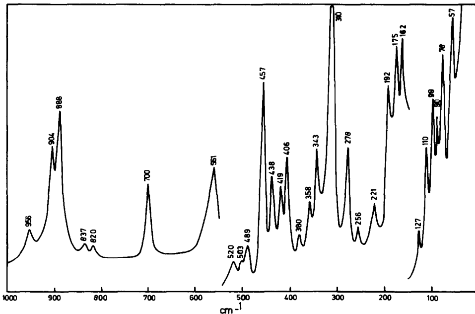
FIG. 3. Raman spectrum of \text{Pb}_2\text{Sc}_2\text{Si}_2\text{O}_9 .
