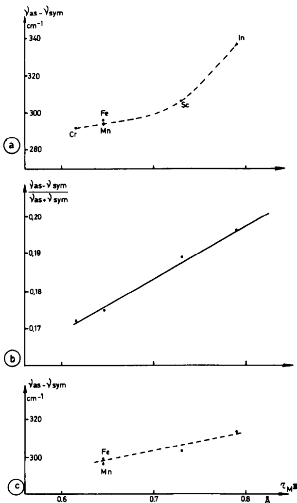
FIG. 4. Relationship between the ionic radius of M^{III} and (a) the difference \nu_{as} - \nu_{sym} , (b) the ratio \nu_{as} - \nu_{sym} / \nu_{as} + \nu_{sym} for the silicates Pb_2M_2^{III}Si_2O_9 , and (c) the difference \nu_{as} - \nu_{sym} for the germanates.
